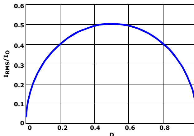
FIGURE 45. I_{RMS}/I_O vs DUTY CYCLE
