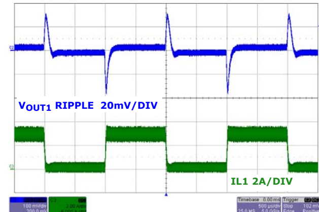
FIGURE 21. LOAD TRANSIENT CHANNEL 1
