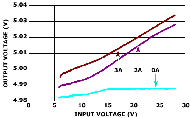
FIGURE 12. OUTPUT VOLTAGE REGULATION vs V_{IN} , CHANNEL 1, T_A = +25^{\circ}C , 5V_{OUT} , F_{SW} = 500kHz
