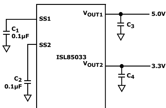
FIGURE 40. RATIMETRIC START-UP
