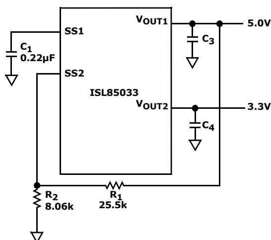
FIGURE 41. ABSOLUTE START-UP
