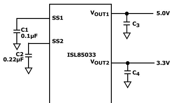
FIGURE 39. INDEPENDENT START-UP
