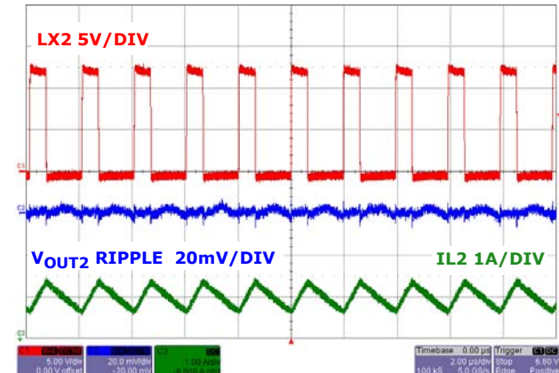
FIGURE 19. STEADY STATE OPERATION WITH FULL LOAD CHANNEL 2
